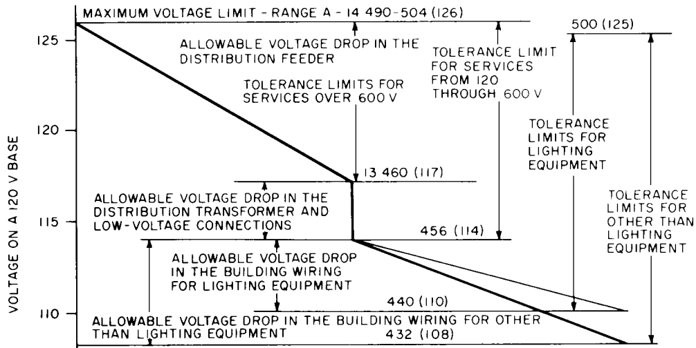
Figure 3-4—Range A voltage profile limits
